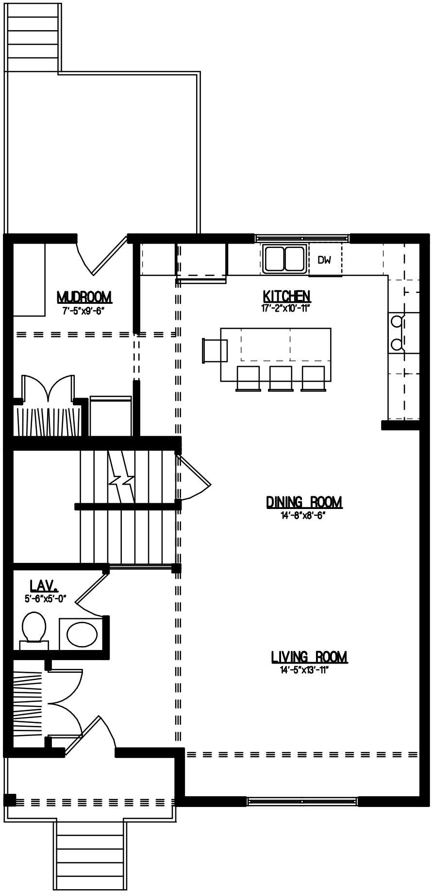
MAIN FLOOR PLAN - 879 SQ. FT.
